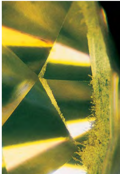
Figure 6. The facet junctions on either side of the upper girdle facets of this 0.59 ct treated green-yellow round brilliant diamond have a frosted, burned appearance that is indicative of heat treatment. Magnified 63 \times .
