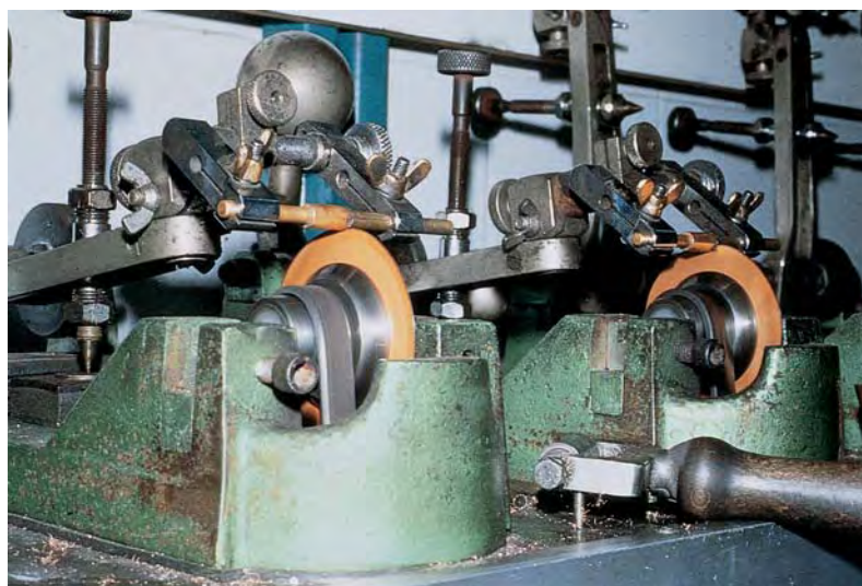
Figure 9. In this photo of a mechanical sawing operation, two machines are shown. The sawing machine controls the lowering of the crystal, attached to a dop, onto a thin copper blade that is revolving at a high speed. Photo by James E. Shigley.
