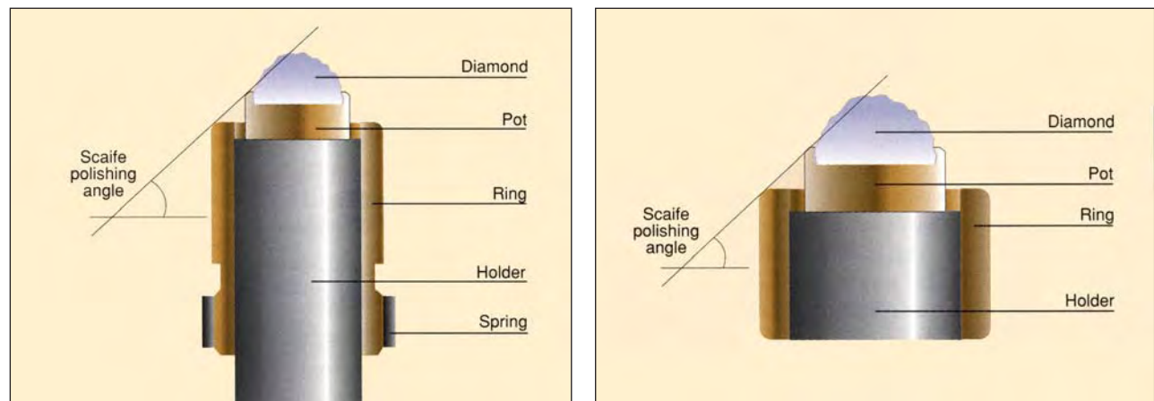
Figure 23. This diagram illustrates how a diamond is set in a holder (left, full holder; right, upper part) for automatic polishing. The angle for polishing the 16 lower-girdle facets is indicated. When the ring comes into physical contact with the scaife, and electrical contact is made, the computer automatically halts the polishing of that particular facet and moves on to the next. When the 16 half-facets are completed, the angle is lowered by approximately 1^\circ and the eight main pavilion facets are polished. For this procedure, an electrical contact is made (and the computer moves to the next facet) when the pot comes into contact with the scaife.
