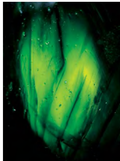
Figure 19. The play-of-color seen in the zircon shown in figure 18 was confined to sharply defined three-dimensional zones, proving that the phenomenon was not due to iridescence from fractures or diffraction from a laminated structure. Magnified 30x.
