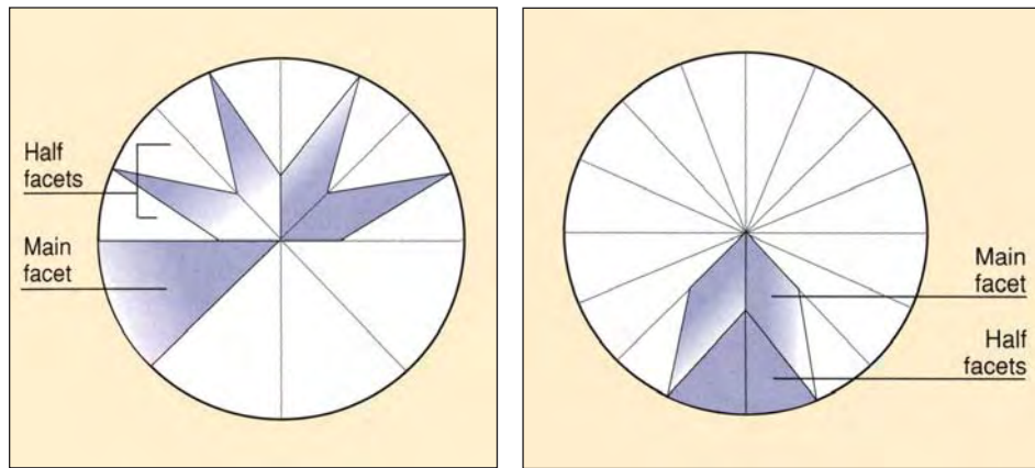
Figure 22. When polishing a diamond by manual methods (left), one first polishes the eight main pavilion facets, and then proceeds to the 16 lower-girdle (half) facets on the pavilion. With automated facet polishing (right), the reverse sequence is followed: the 16 lower-girdle (half) facets of the pavilion are polished first, followed by the eight main pavilion facets.
