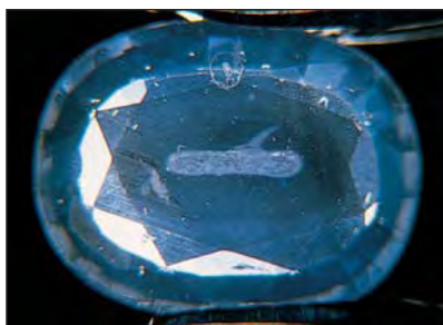
Figure 16. A discoid fracture surrounding a mineral inclusion and the partially exsolved rutile needles prove that this 2.14 ct sapphire was heat treated.
