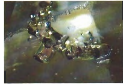
Figure 7. Apatite crystals in korerupine. Magnified 40\times .
