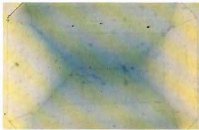
Figure 16. Color zoning in a diffusion-treated synthetic sapphire. Magnified 6x.
