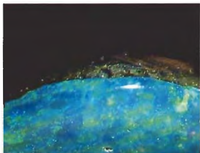
Figure 10. Hemispherical cavities in the cement layer of an opal doublet. Magnified 12 \times .
