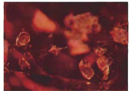
Figure 19. Common inclusions in natural spinel. Dark-field illumination, magnified 30x.
