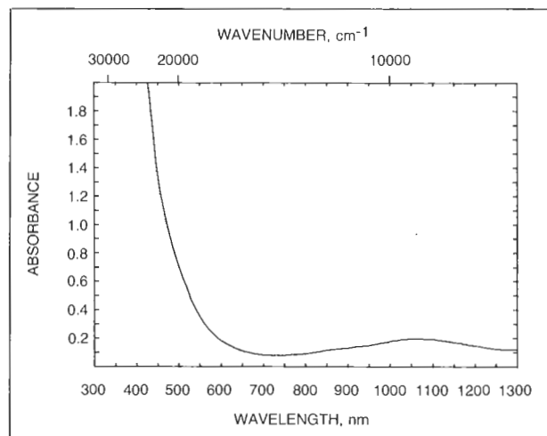
Figure 2. Optical absorption spectrum of orange, irradiated spodumene taken with unpolarized light through a 1.2-cm path.
