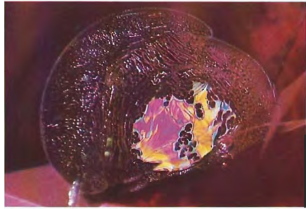
Figure 7. The lace-like pattern of this healing fracture in a Thai ruby under dark-field conditions is given additional life in the form of a brightly colored thin film. The thin-film interference colors resulted from the application of the pinpoint illuminator in an oblique position. Magnified 45 \times .
