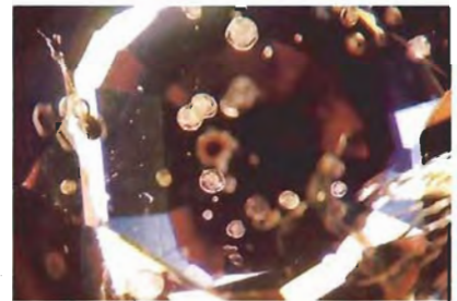
Figure 18. Negative "crystals" in natural spinel. Dark-field illumination, magnified 30x.
