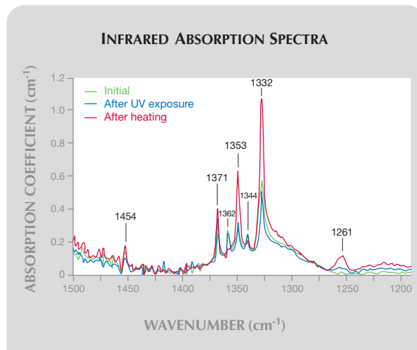
Figure 4. The IR spectra in the region between 1500 and 1200 cm -1 recorded from CVD synthetic diamond sample 11 reveal changes in the strengths of the 1344 (N S 0 ) and 1332 (N S + ) cm -1 peaks, and variations in the strengths of the peaks at 1371, 1362, and 1353 cm -1 . Spectra are shown for the sample in its initial (stable) state, after UV exposure, and after heating.
