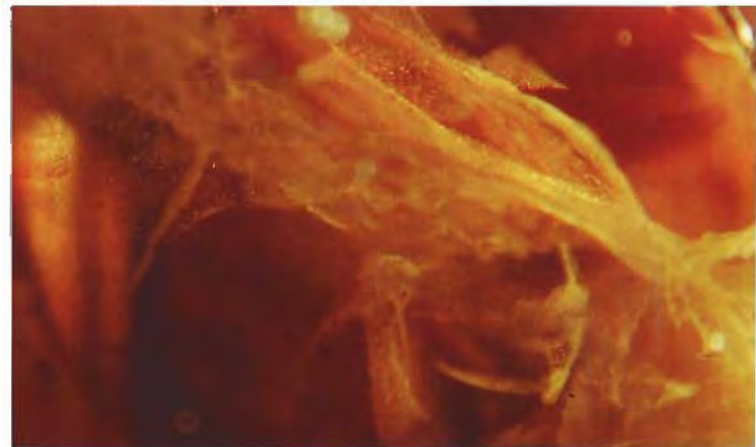
Figure 19. Residual flux takes the form of wispy veils in this Russian synthetic alexandrite. Fiber-optic illumination, magnified 70 \times .
